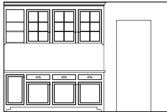
3 KITCHEN ELEVATION SCALE: 3/4" = 1'-0"
